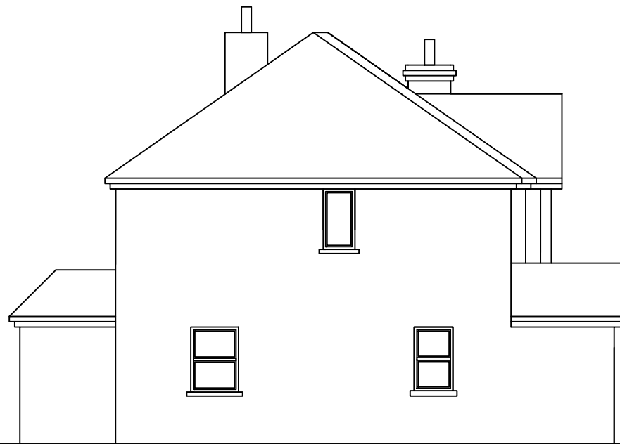
North Elevation
