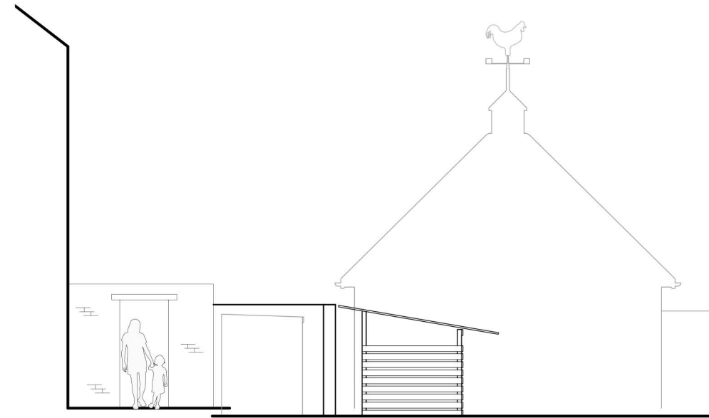
West Elevation as Existing 1:100
