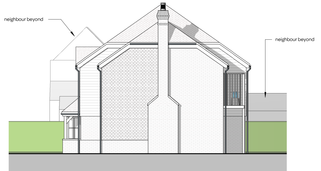
Proposed Side Elevation South East 1:100
