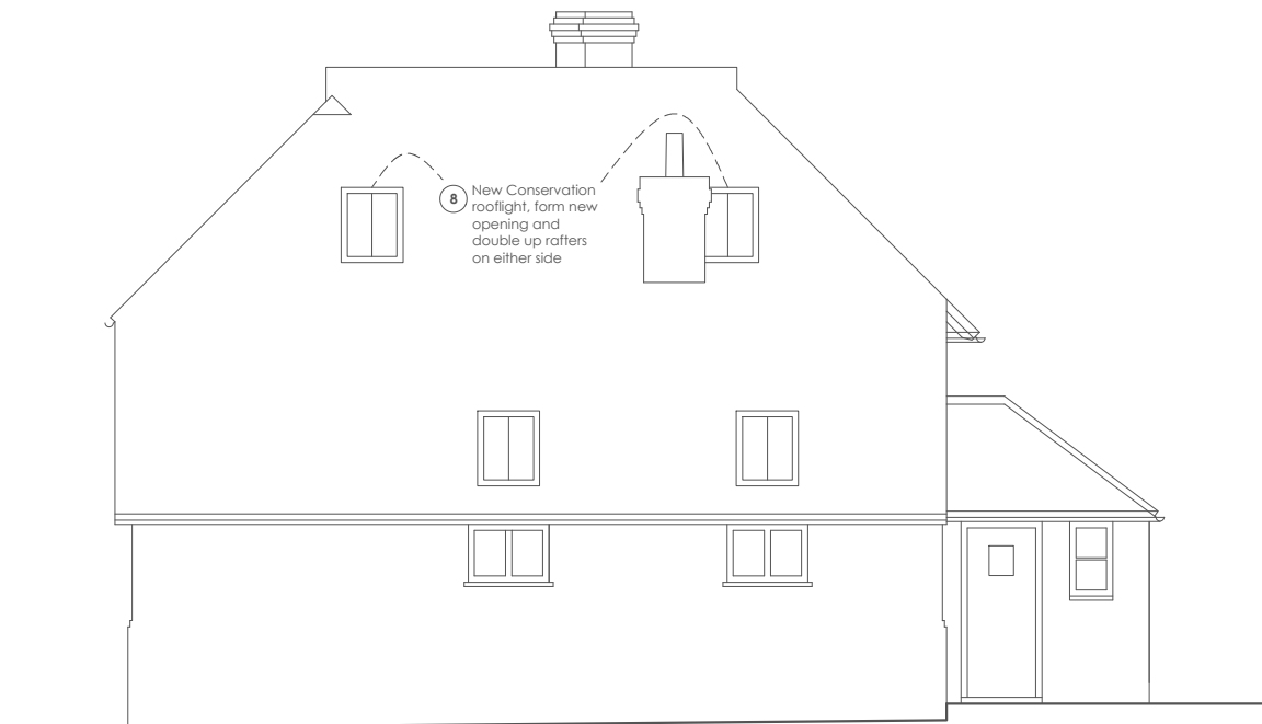
Rear (West) Elevation
