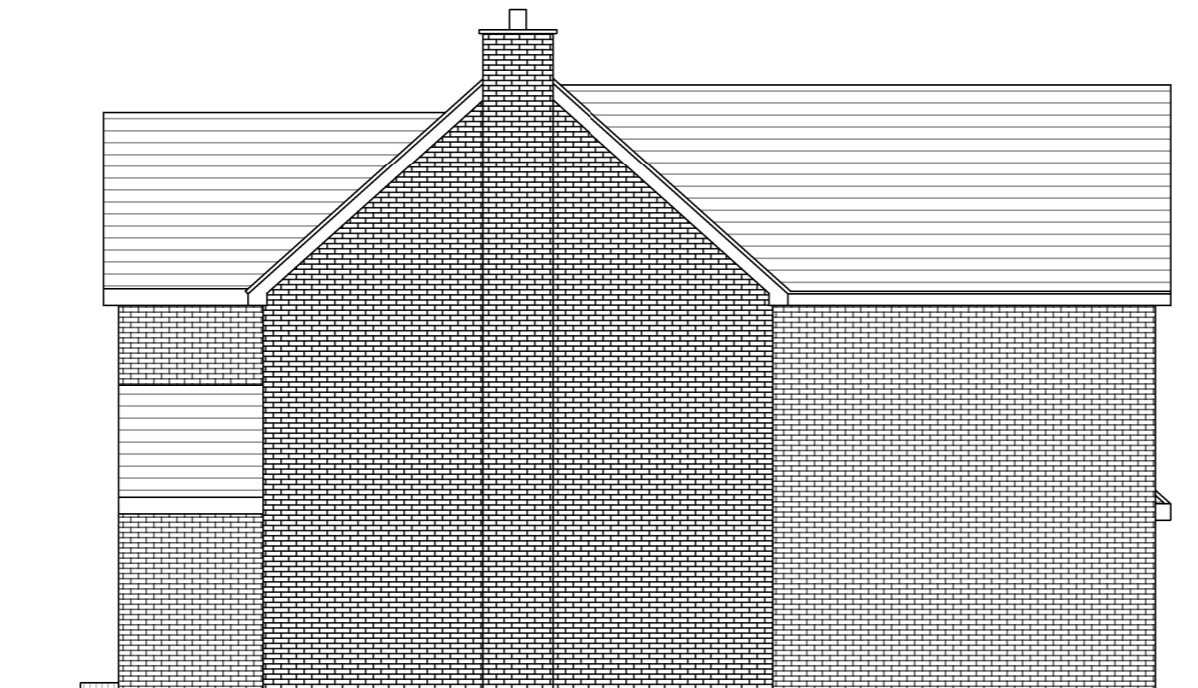
Existing Left Elevation
