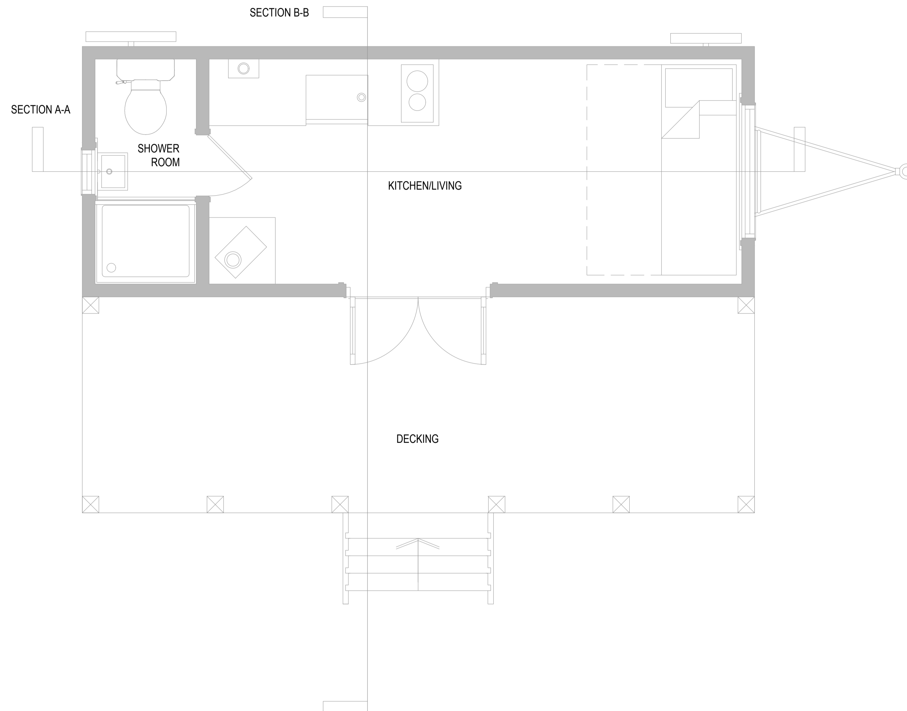
PROPOSED FLOOR PLAN Scale 1:20
