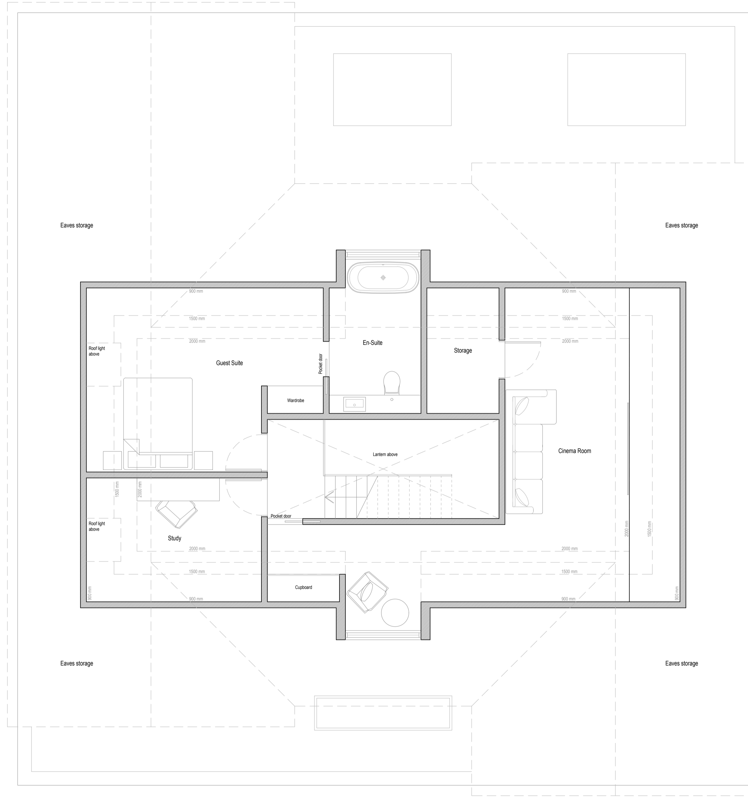
Second Floor Plan (As Built) Scale 1:50
