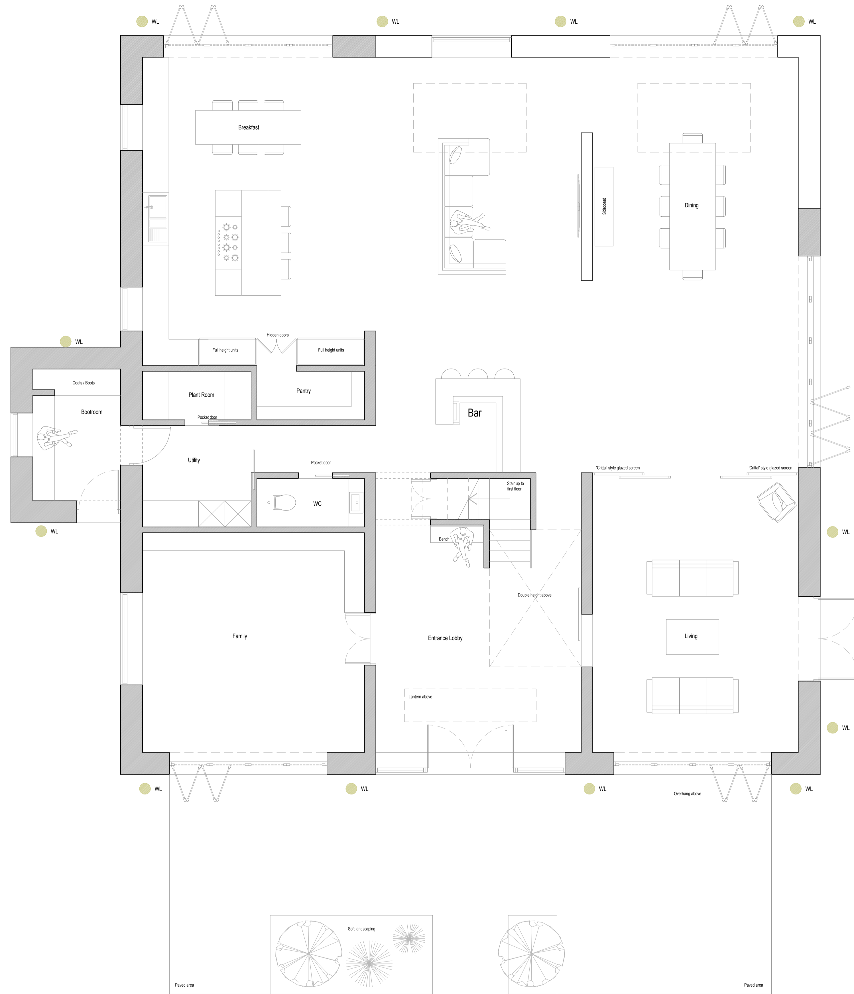
External Ground Floor Lighting Plan Scale 1:50
