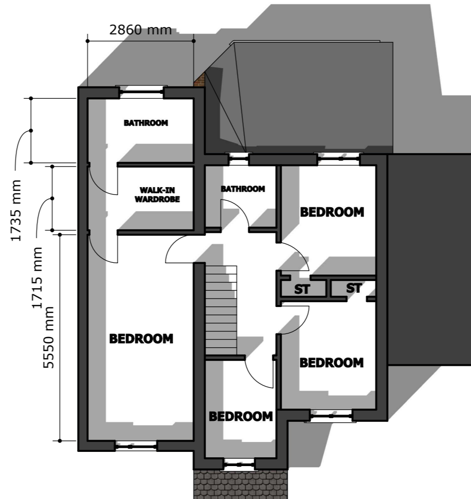
PROPOSED FIRST FLOOR PLAN SCALE 1:100 @ A3
