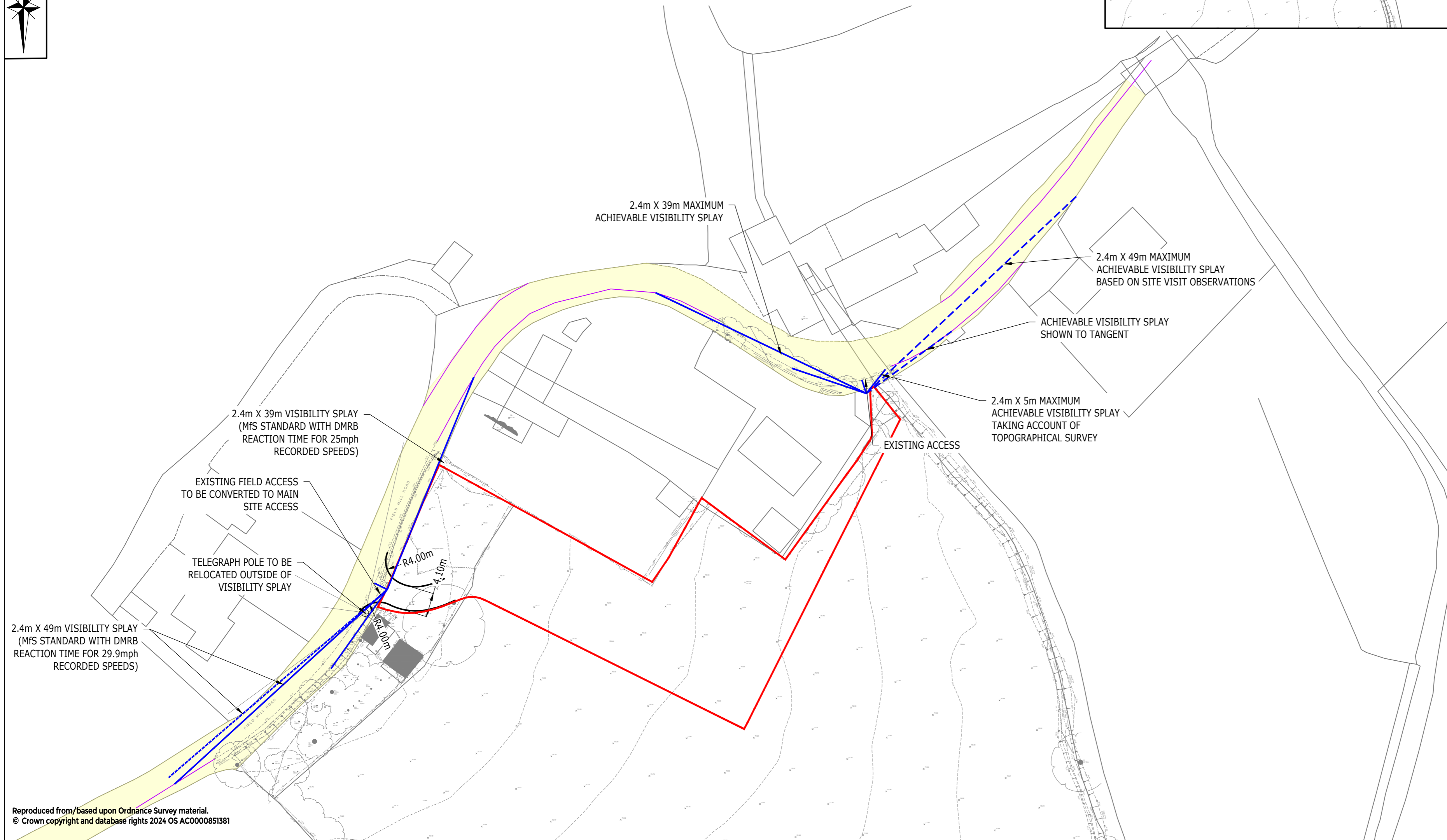
SITE ACCESS AND VISIBILITY SPLAYS SCALE- 1:500
