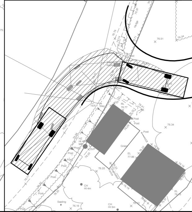
7.5t PANEL VAN LEFT TURN OUT OF PROPOSED ACCESS SCALE - 1:250
