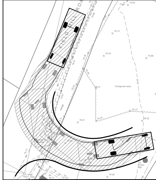
SITE ACCESS AND VISIBILITY SPLAYS SCALE- 1:500
