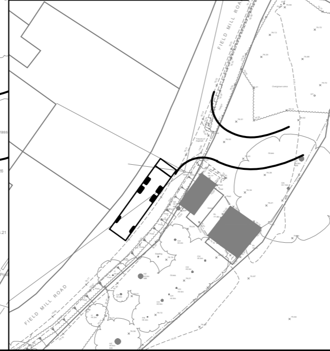
REFUSE VEHICLE STOPPING ON-STREET SCALE- 1:500
