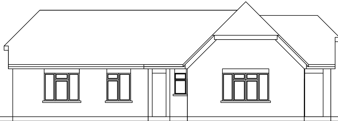
South Elevation
