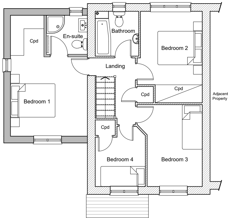
Proposed First Floor Plan - Option 1
